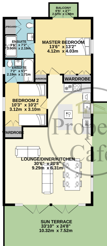
GROUND FLOOR 904 sq.ft. (84.0 sq.m.) approx.
