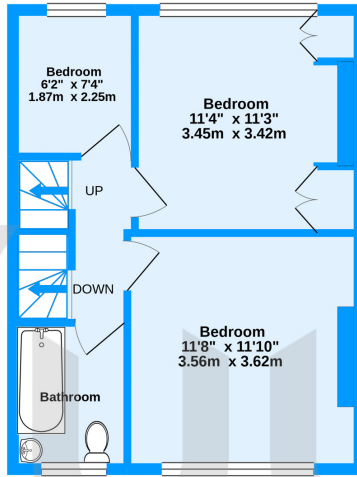
1st Floor 394 sq.ft. (36.6 sq.m.) approx.
