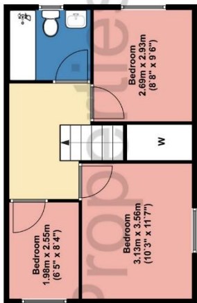
First Floor Approx 37.00 Sq meters (398.00 Sq feet).
