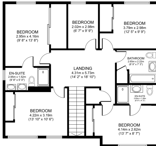
FIRST FLOOR FLOOR AREA 91.3 SQ.M. (982 SQ.FT.) APPROX
