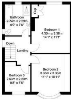
First Floor 45 sq m/484.37 sq ft Approx.
