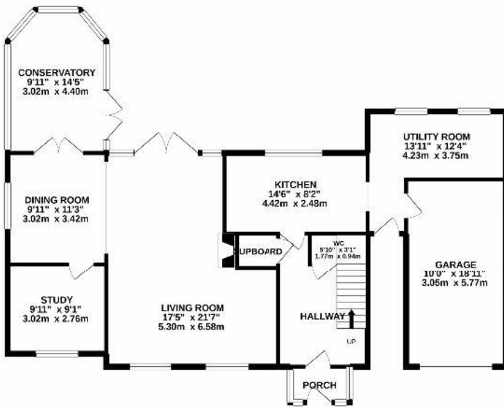
GROUND FLOOR 1227 sq.ft. (114.0 sq.m.) approx.
