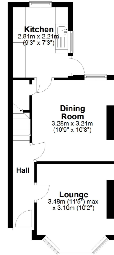
Ground Floor Approx. 31.4 sq. metres (338.4 sq. feet)
