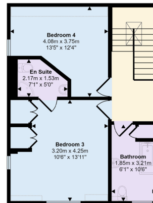
Second Floor Approx 50 sq m / 536 sq ft
