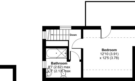
FIRST FLOOR 2
