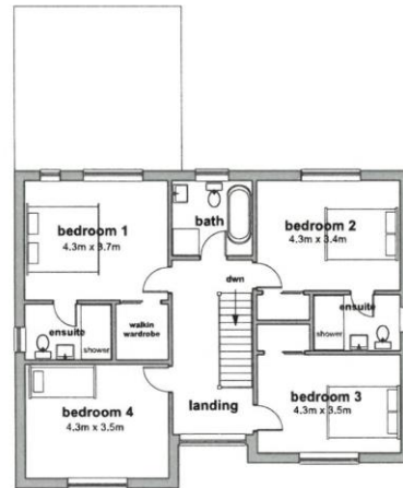
First Floor Plan 1:100
