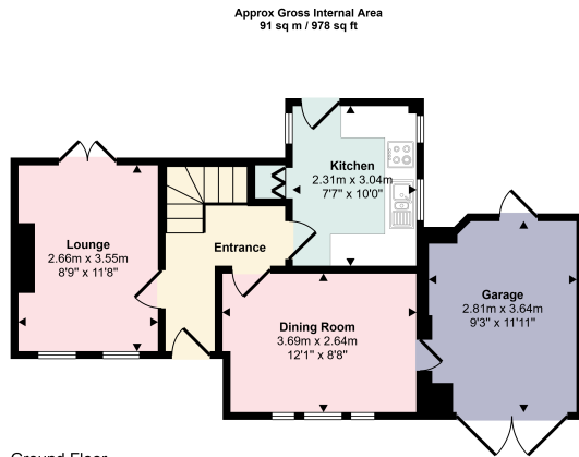
Ground Floor Approx 44 sq m / 477 sq ft
