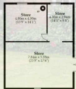
Outbuilding Approx. 76.3 sq. metres (821.1 sq. feet)
