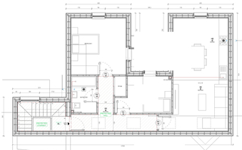
Proposed Floorplan for Top Floor Maisonette (2-Bedroom with Balcony)
