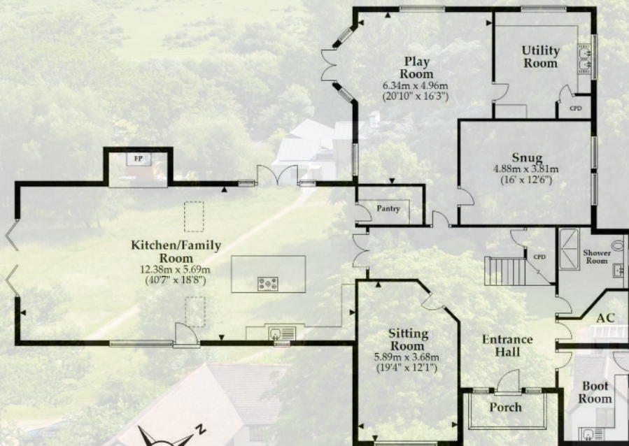
Ground Floor Approx. 214.2 sq. metres (2305.9 sq. feet)
