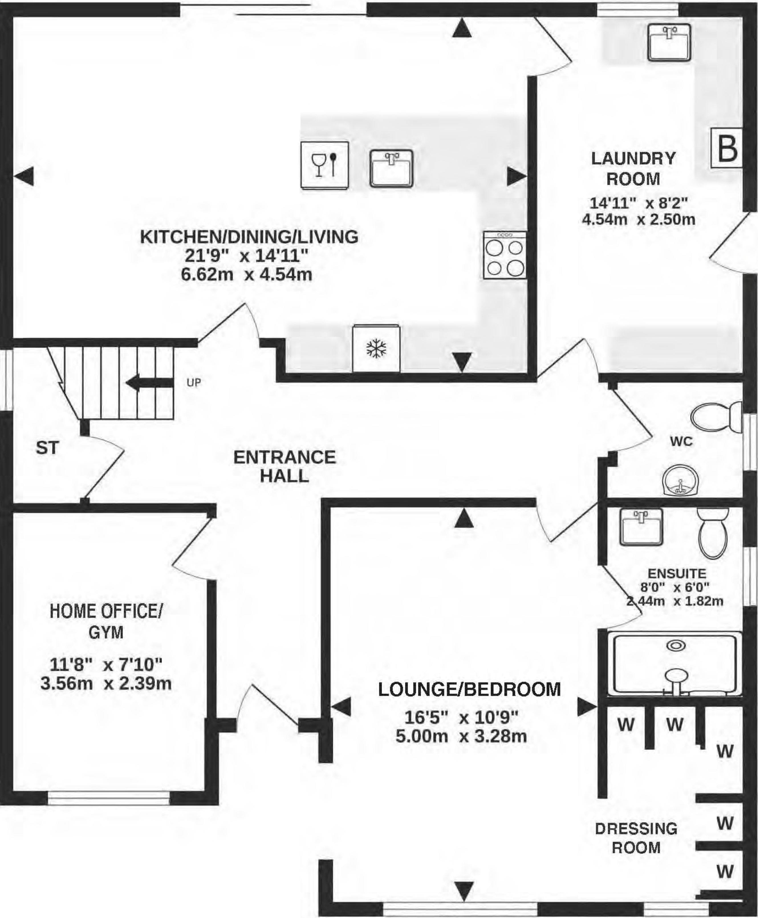
GROUND FLOOR
