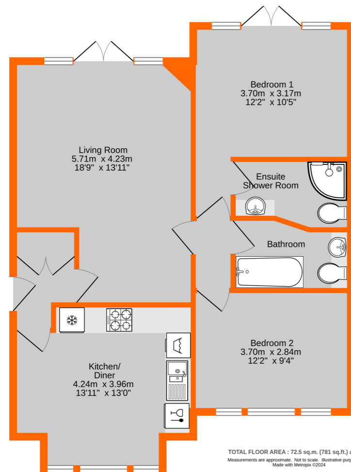
Ground Floor Flat 72.5 sq.m. (781 sq.ft.) approx.
