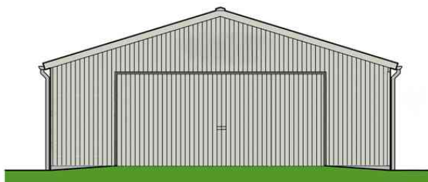
WEST ELEVATION
