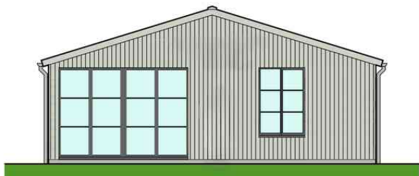
EAST ELEVATION
