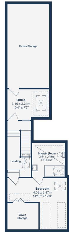
Second Floor Area: 34.0 m 2 ... 366 ft 2
