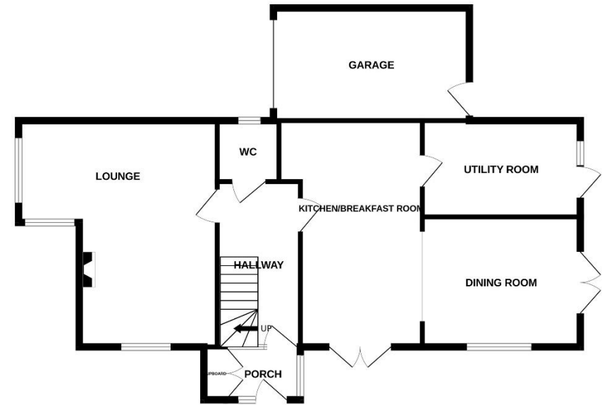
1ST FLOOR
