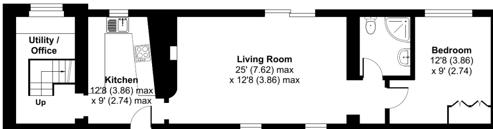
CLARENCE COTTAGE GROUND FLOOR
