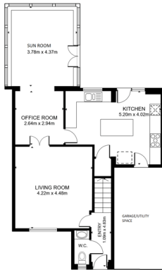
FLOOR 1
