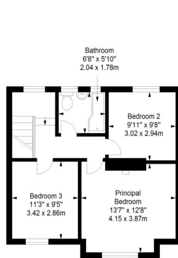
First Floor Approx. 48.2 sq. metres (518.8 sq. feet)
