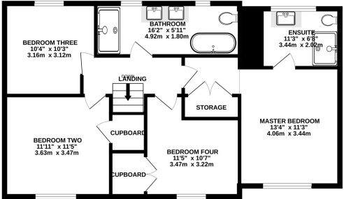
1ST FLOOR 783 sq.ft. (72.7 sq.m.) approx.
