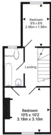
1st Floor Approx. Floor Area 259 Sq. Ft. (24.1 Sq. M.)
