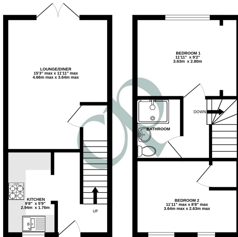
GROUND FLOOR 297 sq.ft. (27.6 sq.m.) approx.
