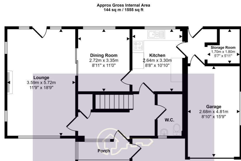
Ground Floor Approx 76 sq m / 814 sq ft
