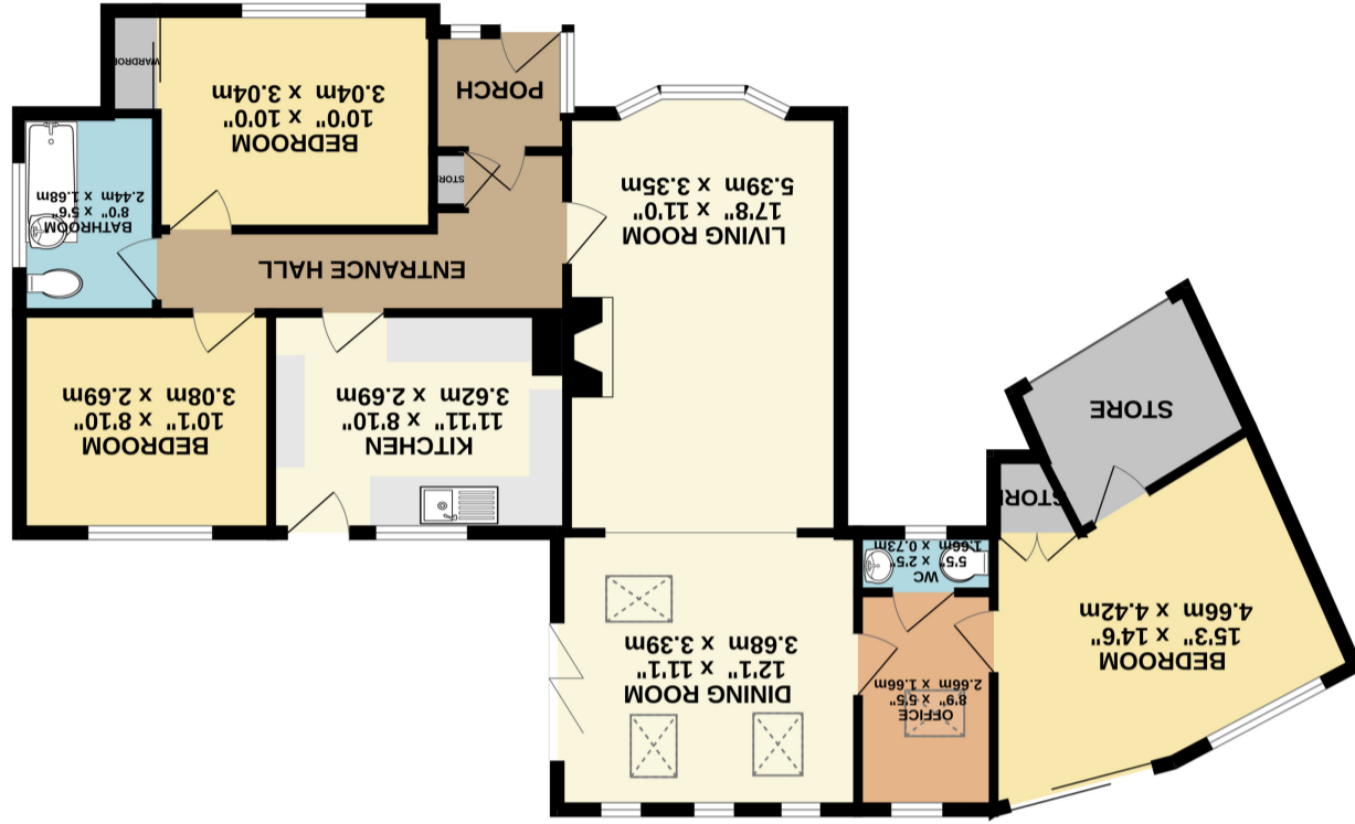
GROUND FLOOR 1019 sq.ft. (94.7 sq.m.) approx.
