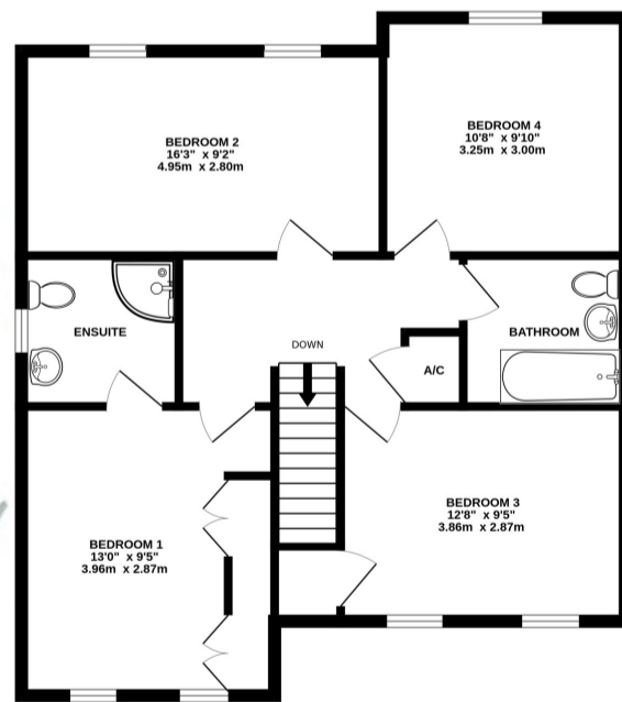
1ST FLOOR 748 sq.ft. (69.5 sq.m.) approx.
