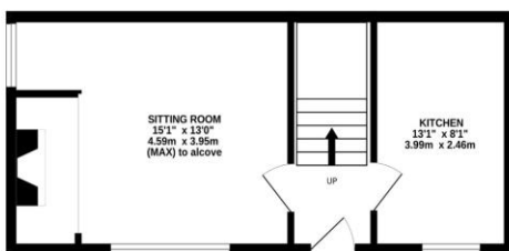
GROUND FLOOR 337 sq.ft. (31.3 sq.m.) approx.
