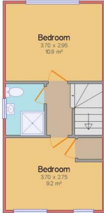
First Floor Gross internal area: 29.0 m 2 (312.6 ft 2 )
