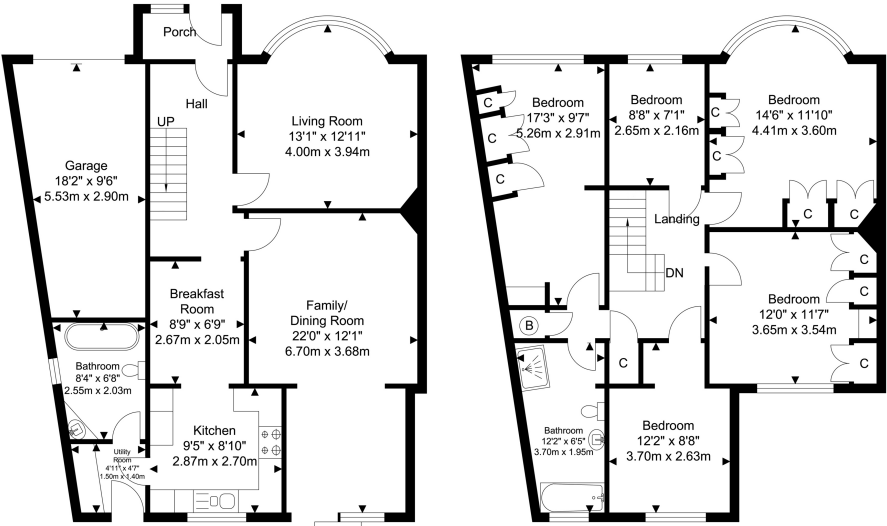
Ground Floor Approximate Floor Area 883.50 SQ.FT. (82.08 SQ.M.)
