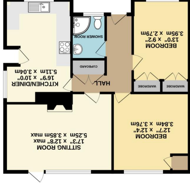
GROUND FLOOR 936 sq.ft. (87.0 sq.m.) approx.
