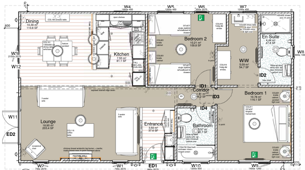
1 01 General Floor Plan 1 : 50
