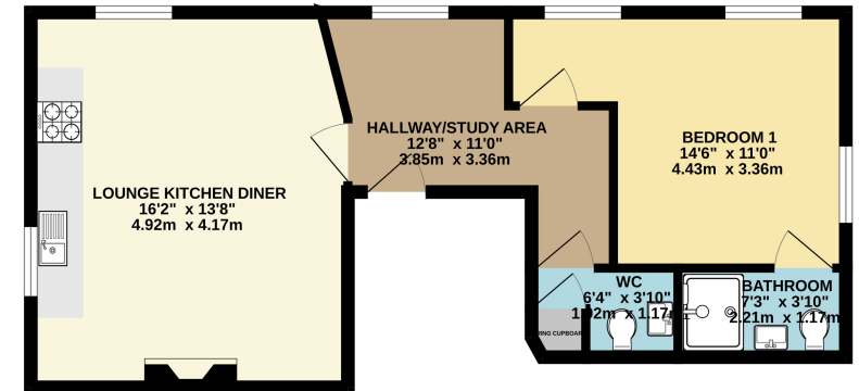
GROUND FLOOR 479 sq.ft. (44.5 sq.m.) approx.
