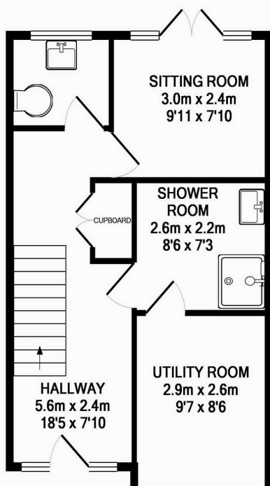
GROUND FLOOR APPROX. FLOOR AREA 36.5 SQ.M. (393 SQ.FT.)
