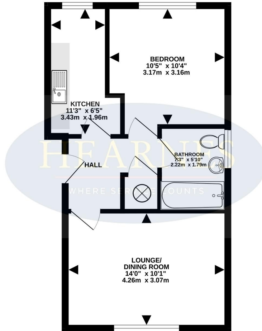
GROUND FLOOR 405 sq.ft. (37.6 sq.m.) approx.
