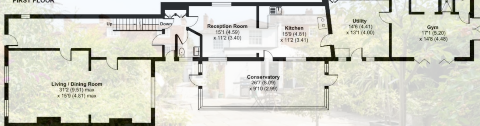
GROUND FLOOR
