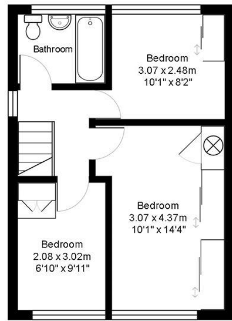
First Floor Area: 34.5 m 2 ... 371 ft 2
