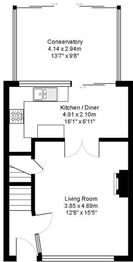
Ground Floor Area: 47.3 m 2 ... 509 ft 2
