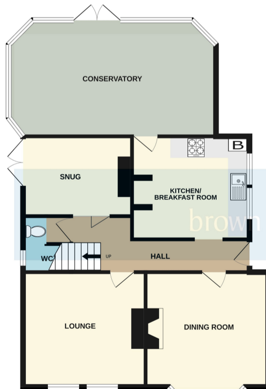
GROUND FLOOR 904 sq.ft. (84.0 sq.m.) approx.
