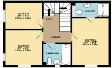
1ST FLOOR 450 sq.ft. (41.8 sq.m.) approx.
