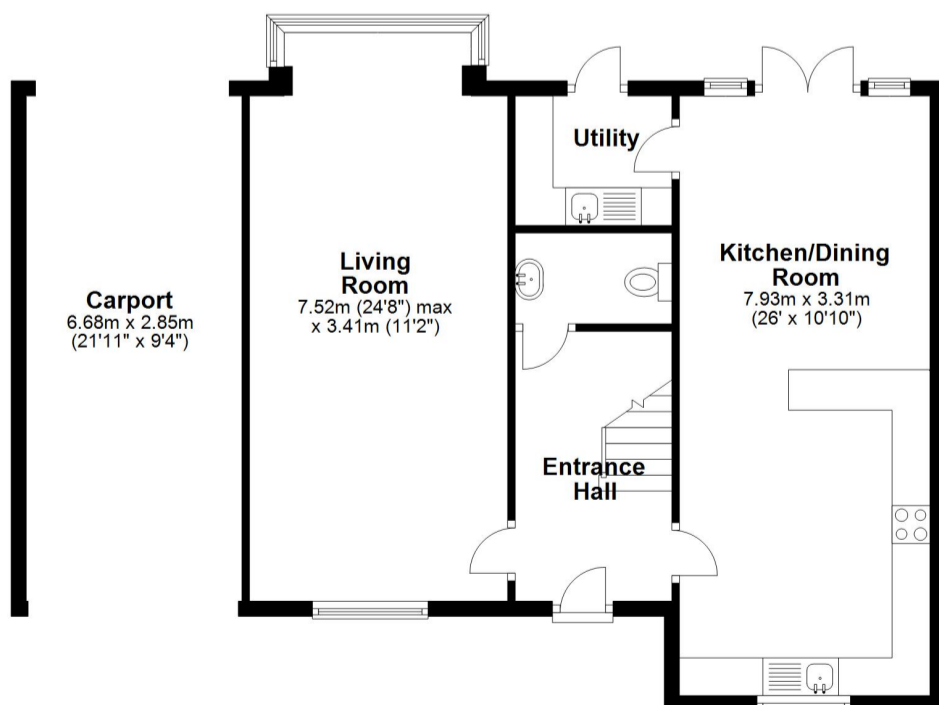
Ground Floor Approx. 86.0 sq. metres (925.5 sq. feet)
