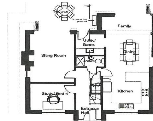
Proposed Ground Floor - 1:100
