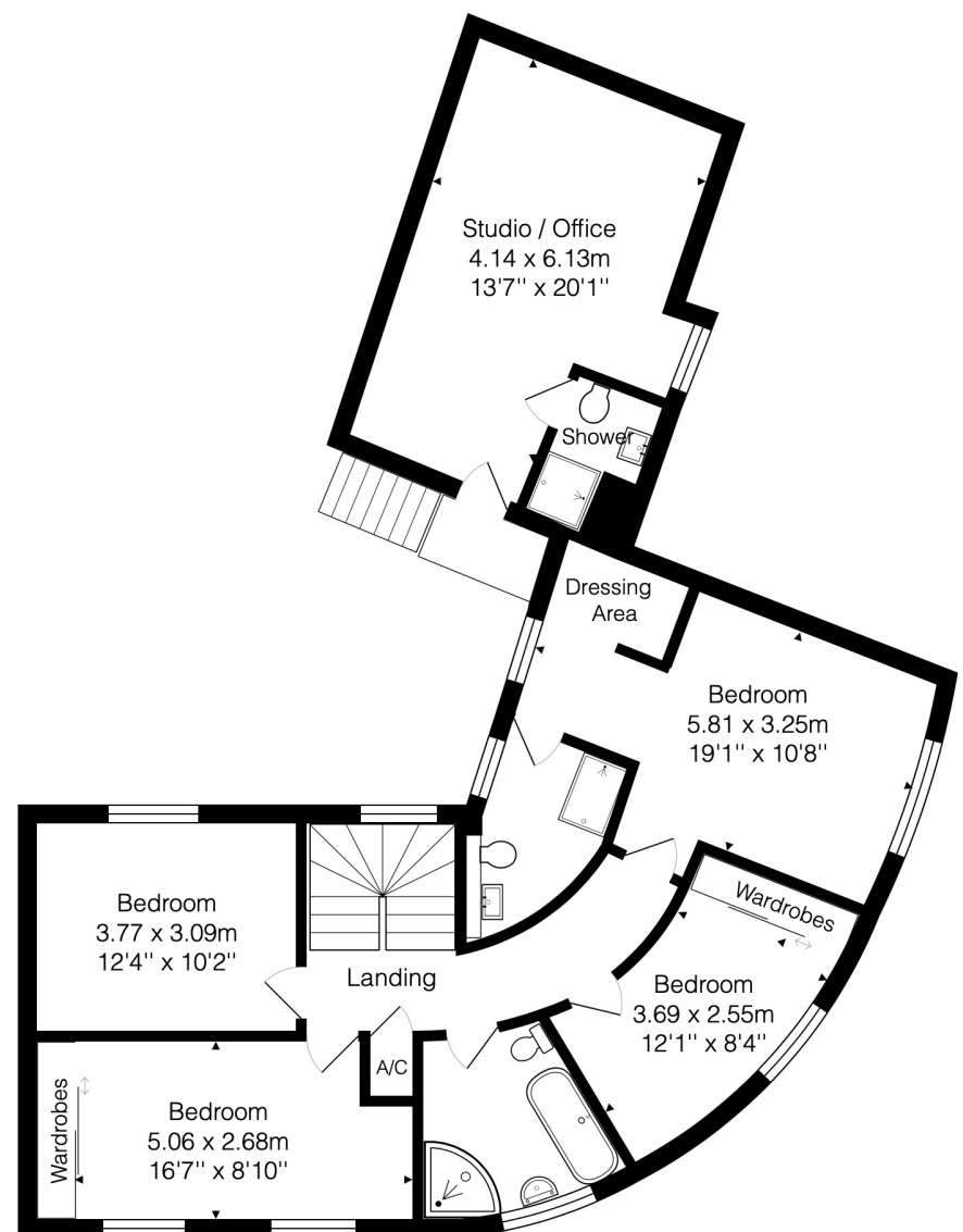
First Floor Area: 107.4 m 2 ... 1156 ft 2
