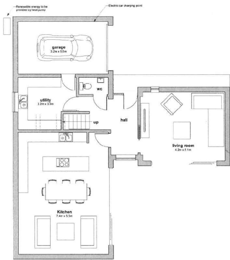
Ground Floor Plan 1:50 0 1.5 3 4.5 6 1:50
