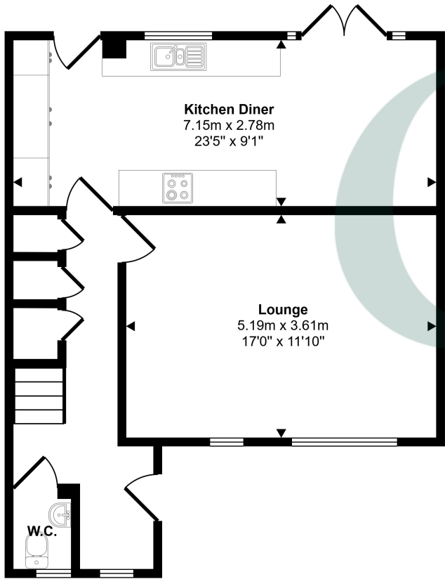
Ground Floor Approx 52 sq m / 562 sq ft
