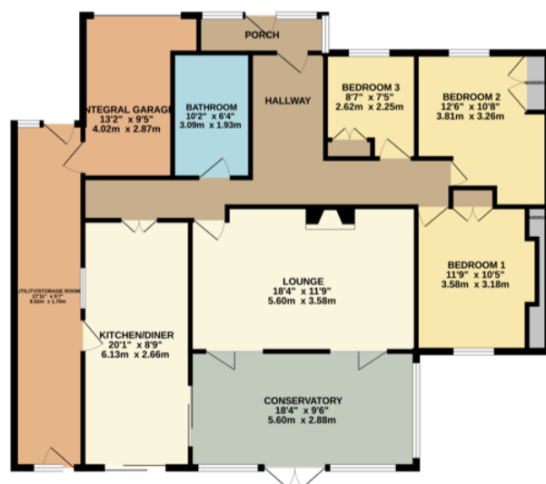
GROUND FLOOR 1382 sq.ft. (128.4 sq.m.) approx.
