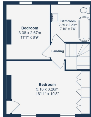
First Floor Area: 34.8 m 2 ... 374 ft 2
