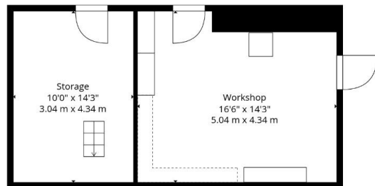
1st Floor
