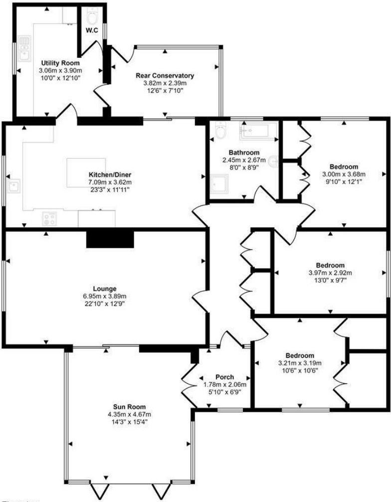
Floorplan
