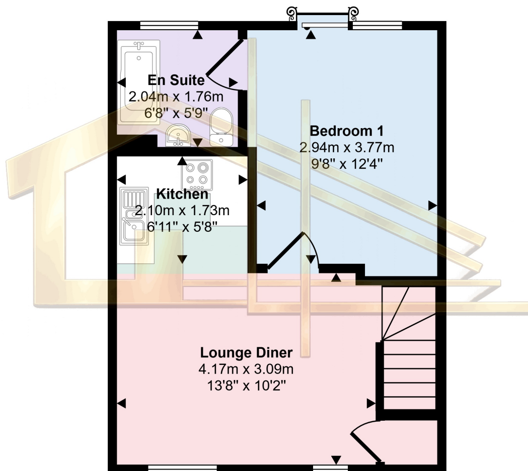
First Floor
